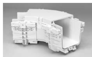
Snap-on Plastic Cover (FGS-SH4E-B shown attached to 45° horizontal elbow with junctions)
