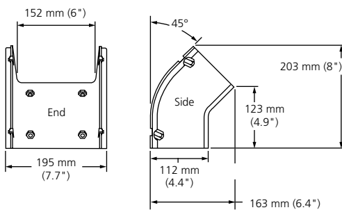
45° Down Elbow (FGS-MD4E-B)
