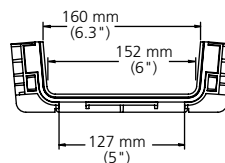
Junction (FGS-JUNC-G)
