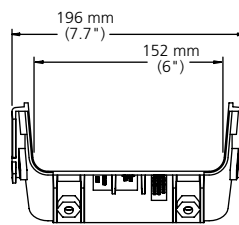
45° Down Elbow (FGS-MD4E-G)
