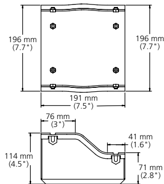
2x6 to 4x6 Adapter (FGS-MDSA-GB)
