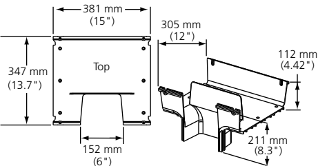
Downspout (FGS-MDSP-F)
