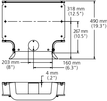
Island T (FGS-ISLAND-F)
