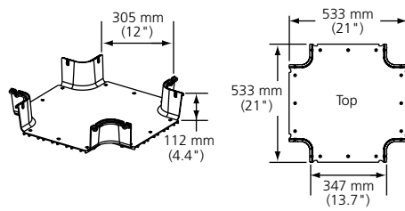
Horizontal Cross (FGS-MHXP-F)
