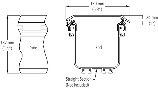
Hinged Cover for 4" Horizontal Straight Section (FGS-MSNC-A)
