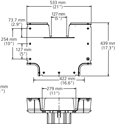
Downspout with Rear T (FGS-MDRT-F)
