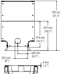
Island T with Single 12" Exit (FGS-ISLAND-H/F)
