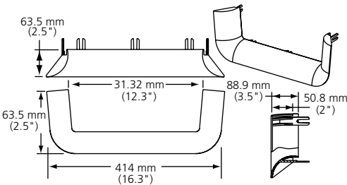
Trumpet Flare (FGS-MTRM-F)
