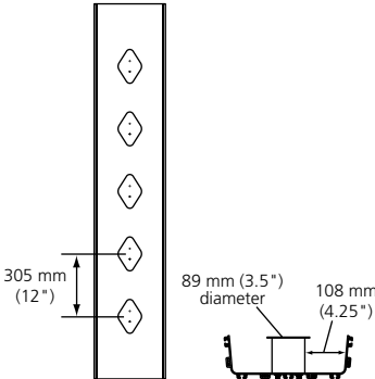
Slack Storage Straight Section (FGS-MSHS-STOR-F)
