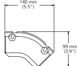
45° Down Elbow (FGS-MD4E-G)
